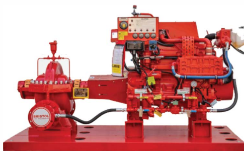
Split Case
